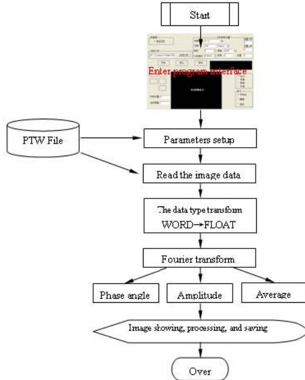
Fig. 3. The flow chart of the Lock-in thermography based on the image sequence processing
