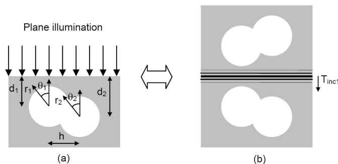
Fig. 1. (a) Geometry of the problem. (b) Equivalent geometry after applying the image theorem.
