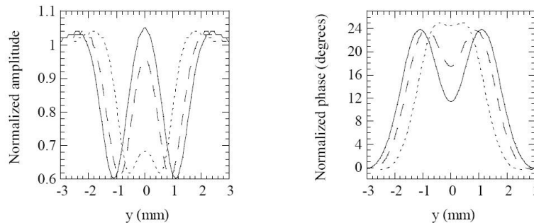
Fig. 2. Amplitude and phase of the surface temperature of two buried cylinders.
