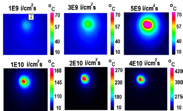
Figure 2: Sequence of infrared images of beam spot on thin graphite targets with increasing beam flux. Each image corresponds to maximum intensity during a pulse, for a 3.6 MeV/u, 4 ms, 38 Hz ^{197}\text{Au} beam.
