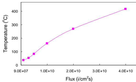
Figure 3: Maximum temperature recorded within the beam spot on thin graphite targets exposed to 3.6 MeV/u ^{197}\text{Au} ions, with increasing beam intensity, as a function of beam flux.
