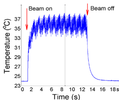
Figure 1: Temporal evolution of temperature within the center of the beam spot during irradiation with 1 \times 10^9 \text{i/cm}^2 \text{s} ^{197}\text{Au} ions with a energy of 3.6 MeV/u, 4 ms pulse length and a repetition rate of 38 Hz.
