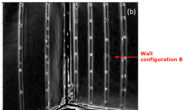
Fig. 7. EOF n°2 with gradient scan for wall configuration B (summer conditions; cooled IR camera; 120/120 minutes of heating and cooling phases; 1170 W)
