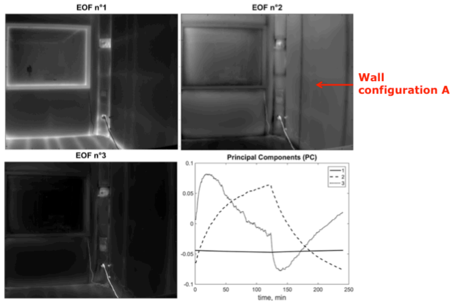
Fig. 6. EOFs n°1 to 3 and their associated Principal Components for wall configuration A (autumn conditions; uncooled micro-bolometer IR camera; 120/120 minutes of heating and cooling phases; 1170 W)
