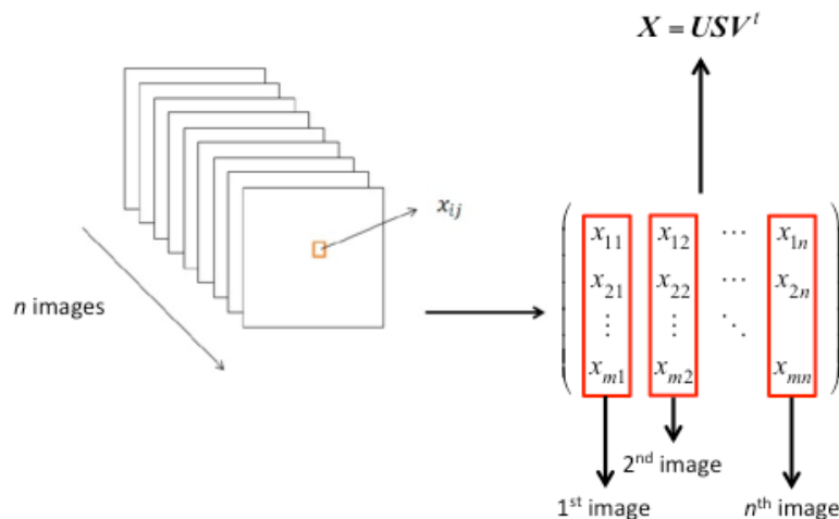
Fig. 5. Rearrangement of the thermographic sequence before application of the SVD treatment
