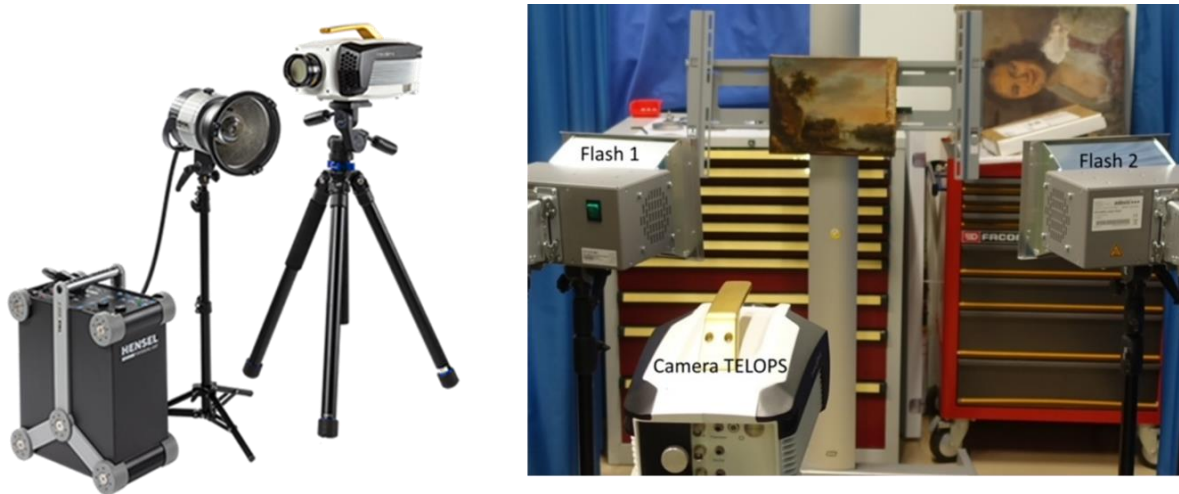
Figure 1. Active thermography set up and experimental configuration including the paintings, TELOPS camera and two flash lamps.
